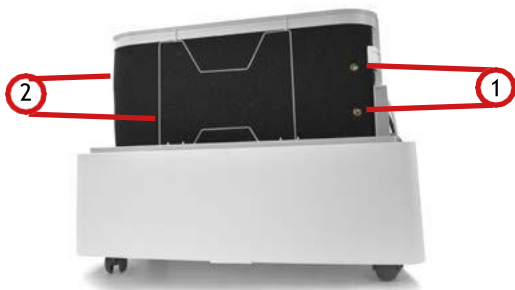
Fig. 6.3.2.3.3: B 600 with activated carbon cleaning filter
